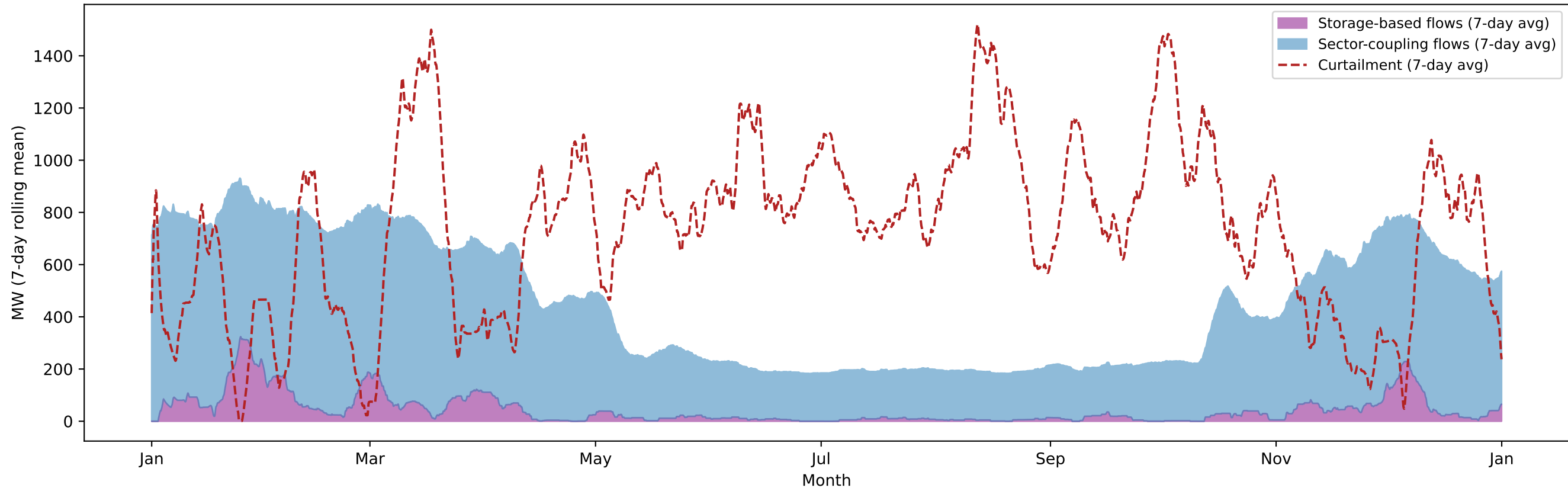
Rolling Weekly Flexibility Intensity Storage-based vs Sector-coupling vs Curtailment
